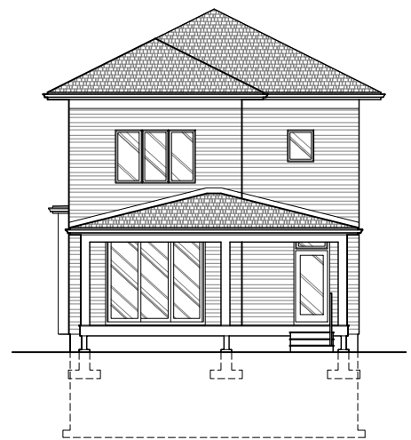
REAR ELEVATION (WEST)
