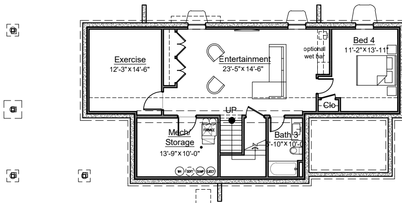
BASEMENT
